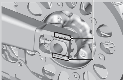
Chain adjuster index marks
